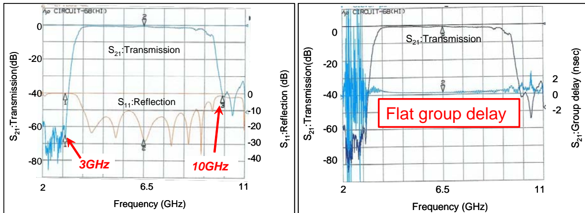
Fig. 1 Measured results of the Ring Filter Transmission and Reflection characteristics.
