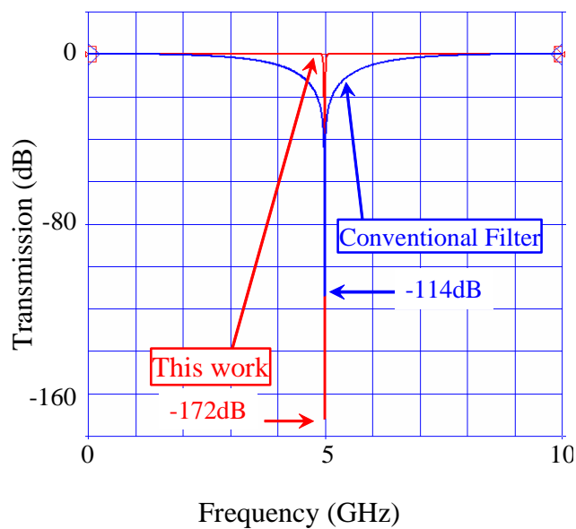
Fig. 2 Measured results of the Ring Filter.
